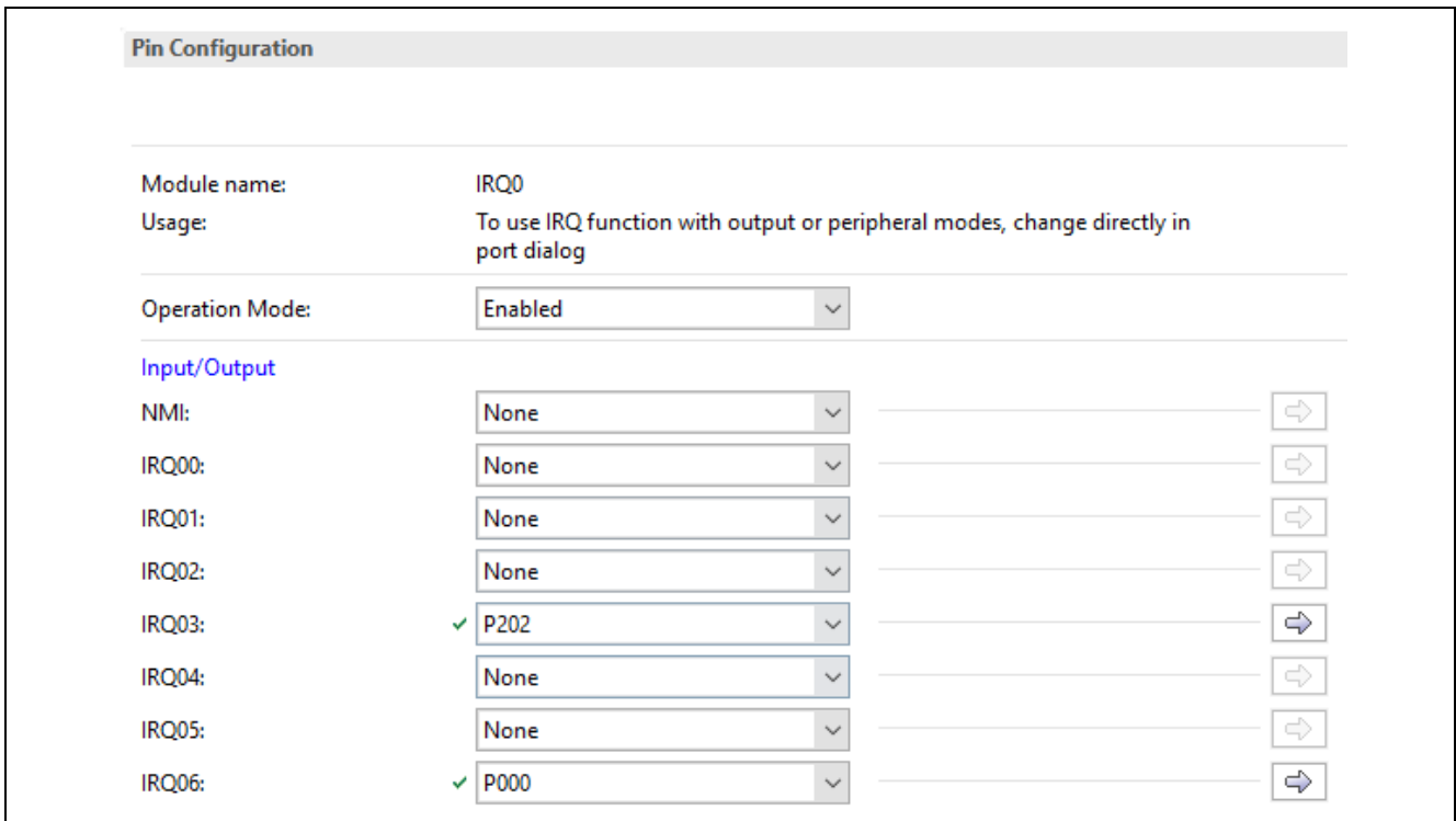
Figure 26. Enable P202, P000 as IRQ03, IRQ06 inputs Respectively using Pin Configurator in Renesas FSP
