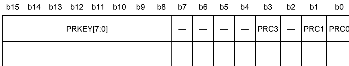
Figure 23. PRCR Register
