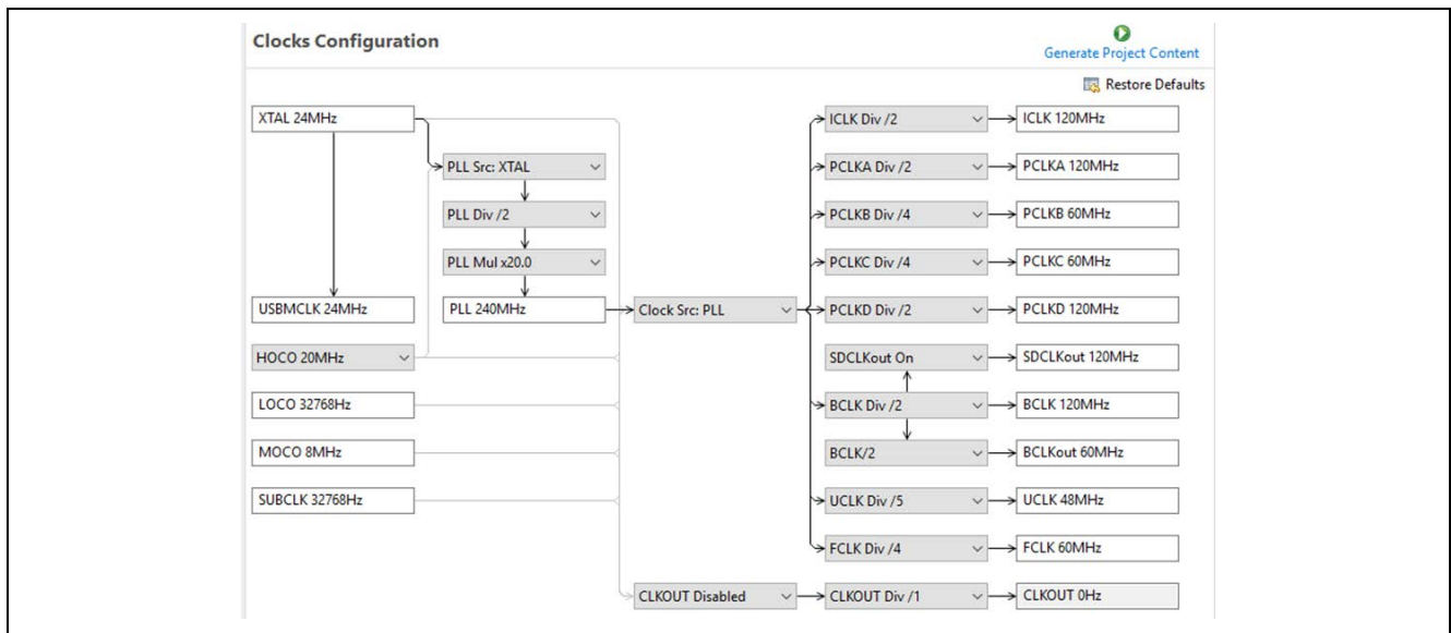
Figure 11. Clock Settings Using Renesas FSP Configurator
