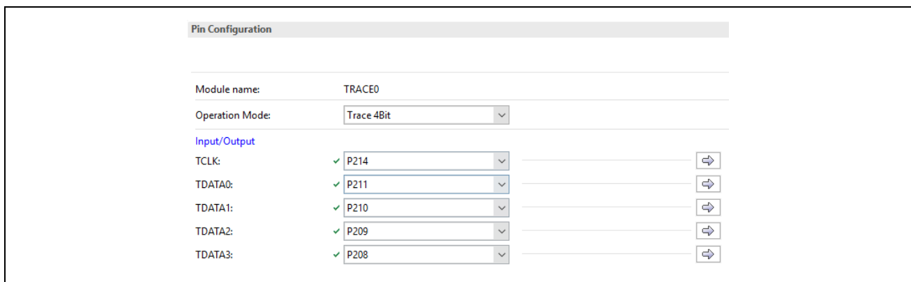
Figure 6. Enabling Trace Ports in Runtime Using FSP Configurator
