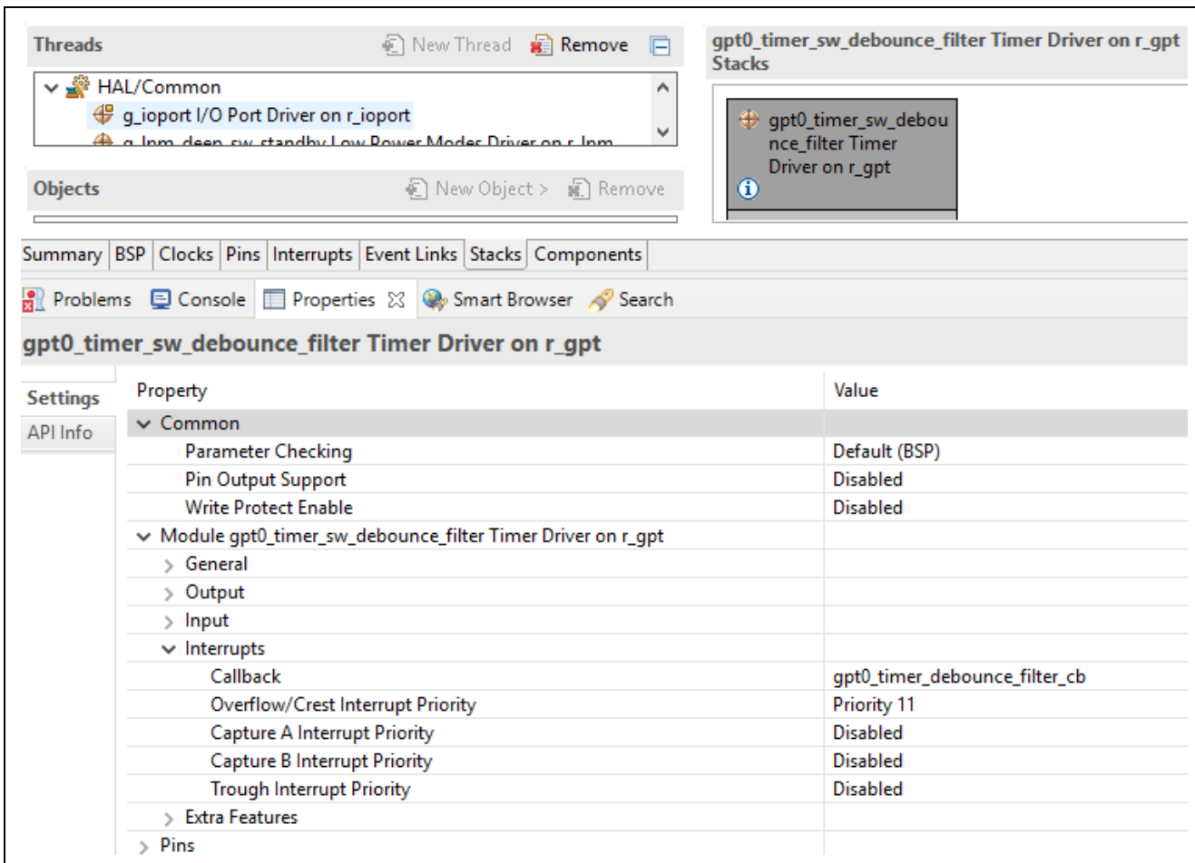
Figure 30. Enable GTP0 Overflow Interrupt and Set User Callback Functions Invoked by Interrupt Service Routine
