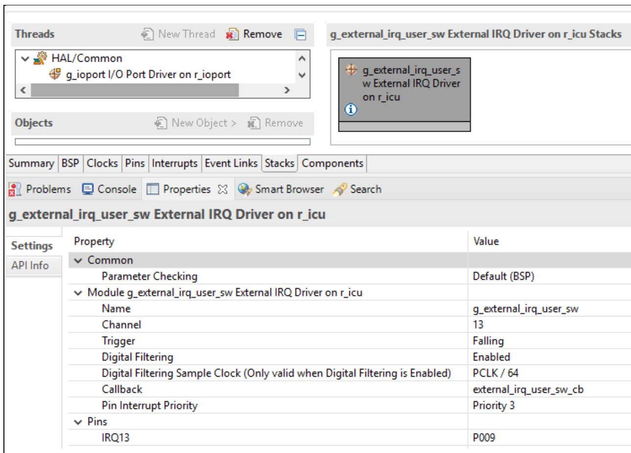
Figure 27. Configure IRQ13 using Renesas FSP Configurator
