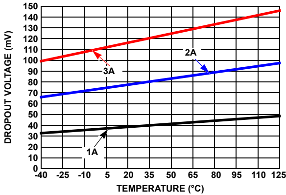
FIGURE 12. DROPOUT VOLTAGE vs TEMPERATURE
