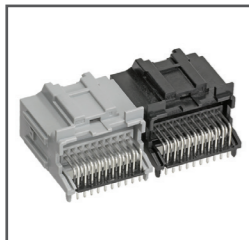
2.54mm (.100") pitch, right angle ganged multi-bay headers, PAP version
