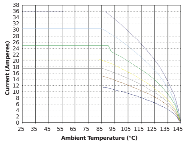
2.80mm Sn Receptacle to Stac64 Header, 10 to 22 AWG USCAR-2 Rev 4
