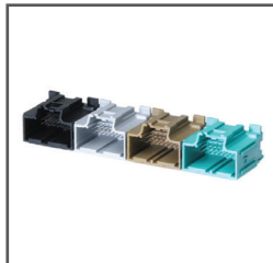
2.54mm pitch vertical ganged multi-bay headers
