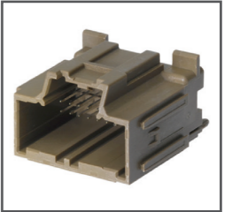
2.54mm (.100") pitch, vertical single-bay signal header
