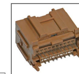
34772 series, vertical single-bay hybrid power header
