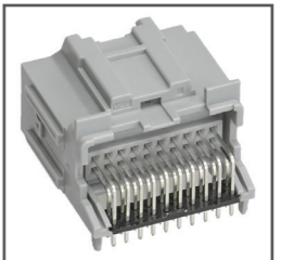
2.54mm (.100") pitch, right angle single-bay signal header, PAP version
