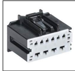
31372 series, 5.25mm (.206") pitch, with TPA, hybrid power receptacle
