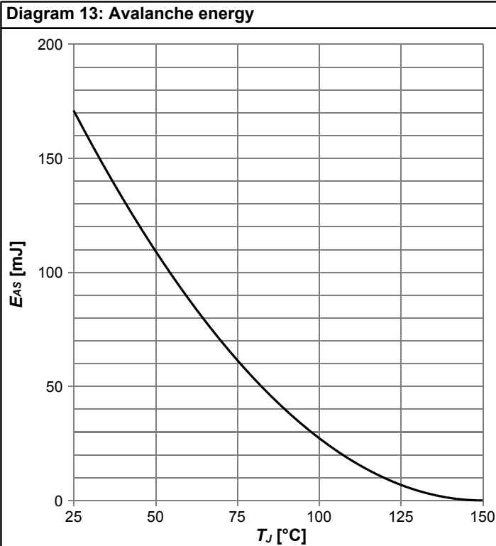
E_{AS}=f(T_J) ; I_D=6.4 A; V_{DD}=50 V
