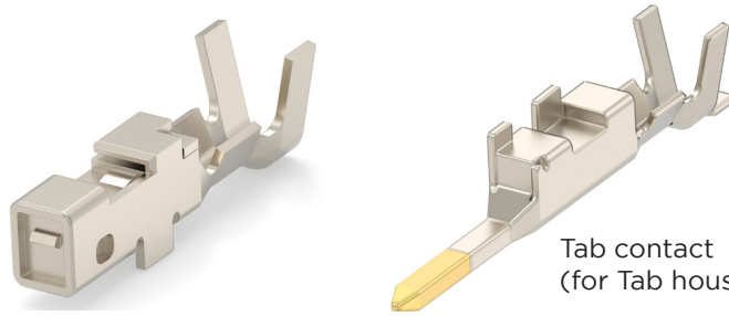
Receptacle Contact (for Receptacle housing)
