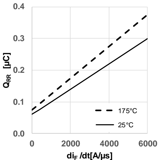
Figure 19 Typical reverse recovery charge as a function of diode current slope ( Q_{rr} = f(di_i/dt) , V_{DD} = 800V , V_{GS} = 0V/18V , I_D = 6A , ind. load, test circuit in Fig.E, body diode at V_{GS} = 0V )
