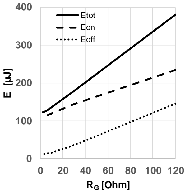
Figure 17 Typical switching energy losses as a function of gate resistance ( E = f(R_{G,ext}) , V_{DD} = 800V , V_{GS} = 0V/18V , I_D = 6A , T_{vj} = 175^\circ C , ind. load, test circuit in Fig. E, diode: body diode at V_{GS} = 0V )
