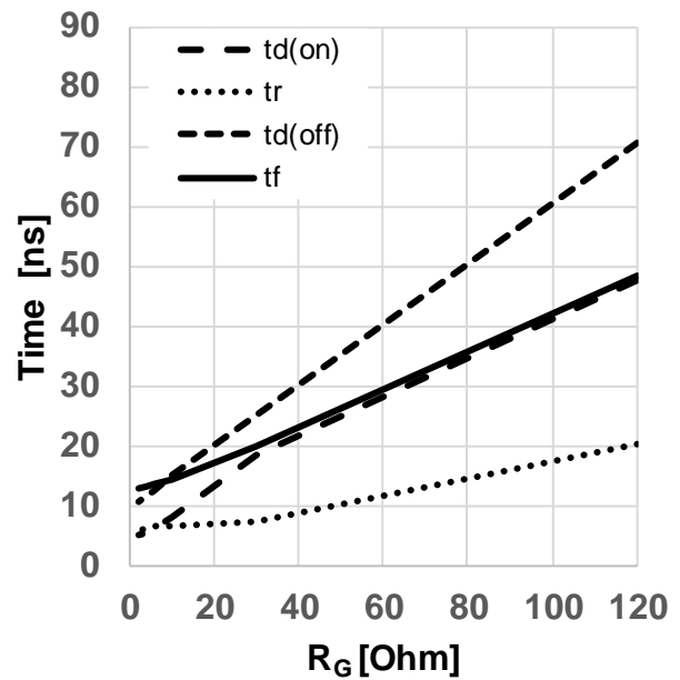
Figure 18 Typical switching times as a function of gate resistor ( t = f(R_{G,ext}) , V_{DD} = 800V , V_{GS} = 0V/18V , I_D = 6A , T_{vj} = 175^\circ C , ind. load, test circuit in Fig. E, diode: body diode at V_{GS} = 0V )
