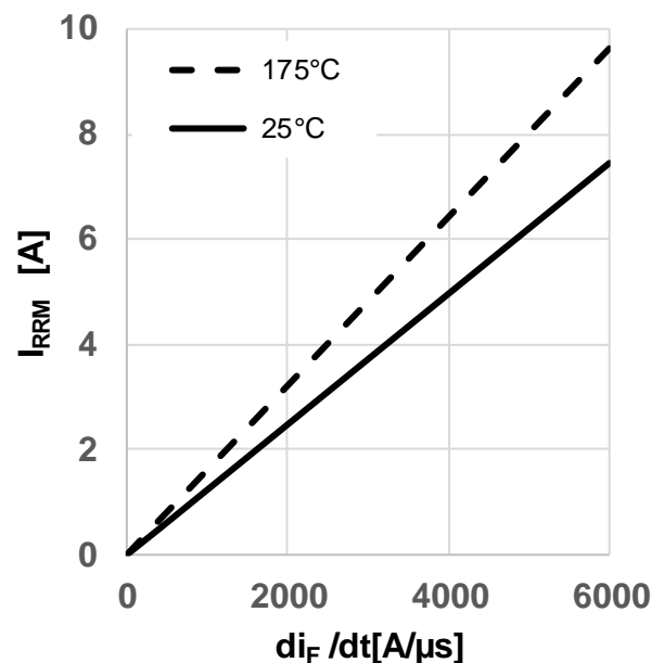
Figure 20 Typical reverse recovery current as a function of diode current slope ( I_{rrm} = f(di_i/dt) , V_{DD} = 800V , V_{GS} = 0V/18V , I_D = 6A , ind. load, test circuit in Fig.E, body diode at V_{GS} = 0V )
