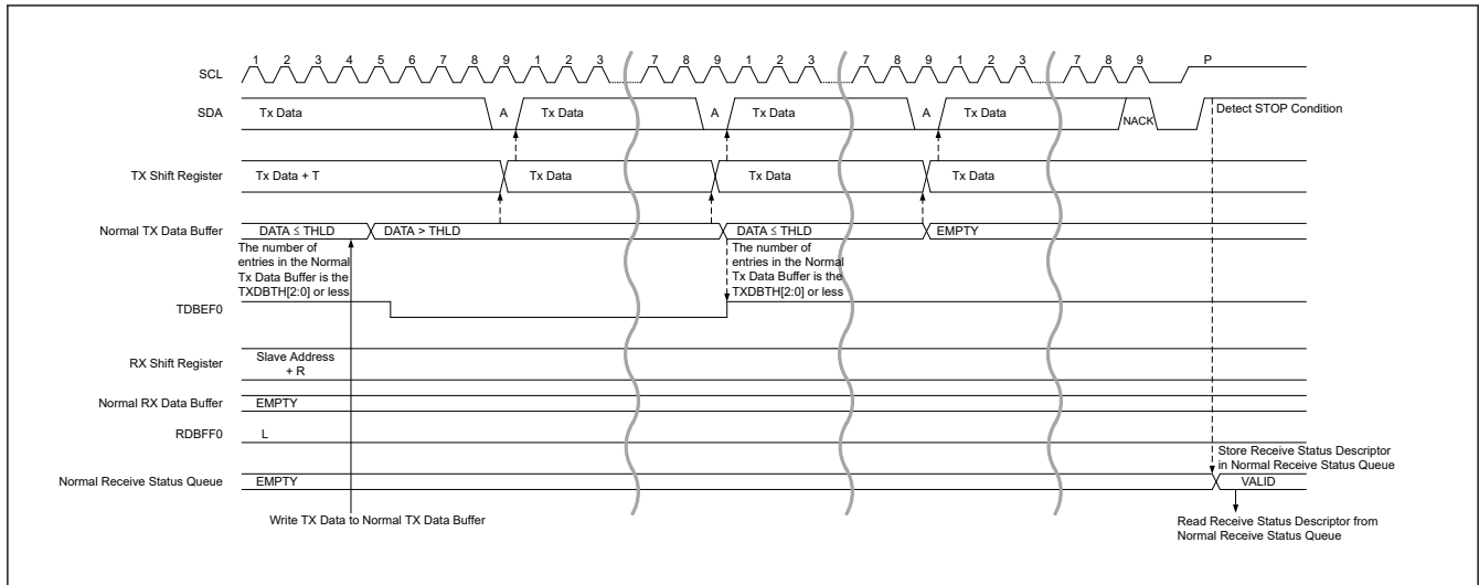
Figure 25.43 Legacy I2C message data read transfer timing (2/2)
