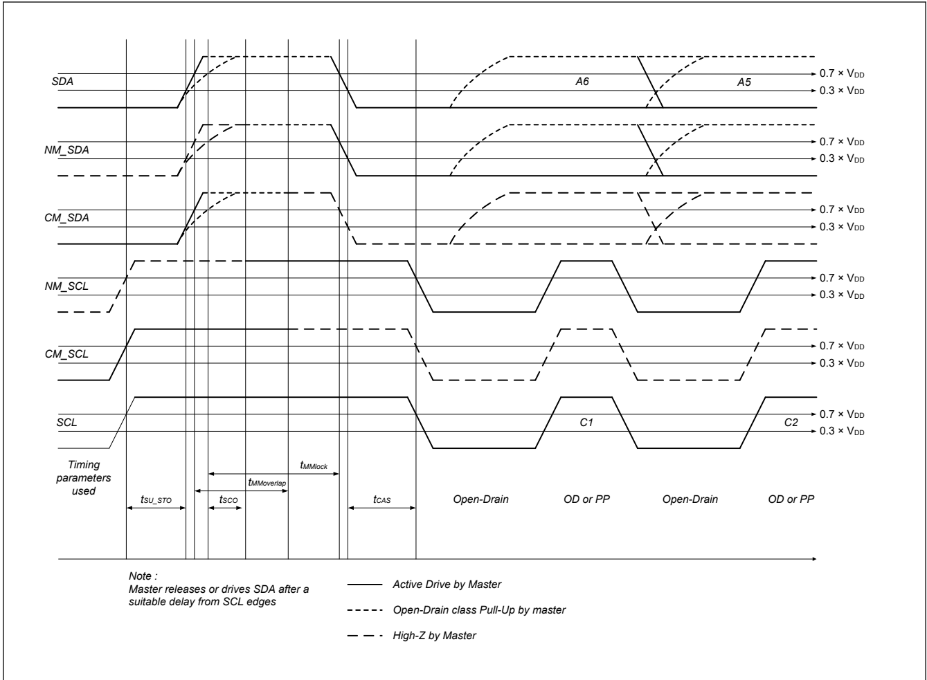
Figure 36.42 I3C Timing
