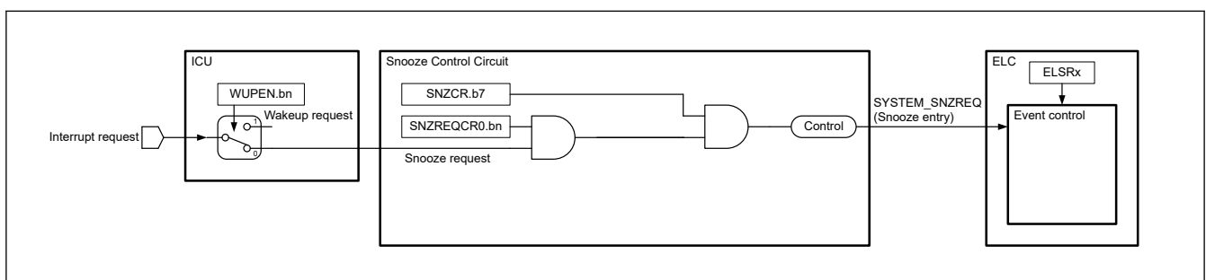
Figure 10.7 Snooze mode entry configuration
