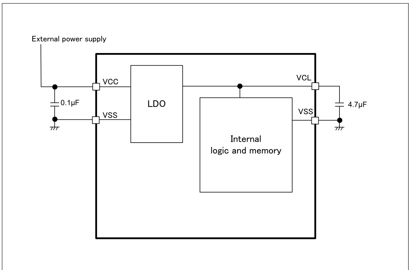
Figure 35.1 LDO mode settings
