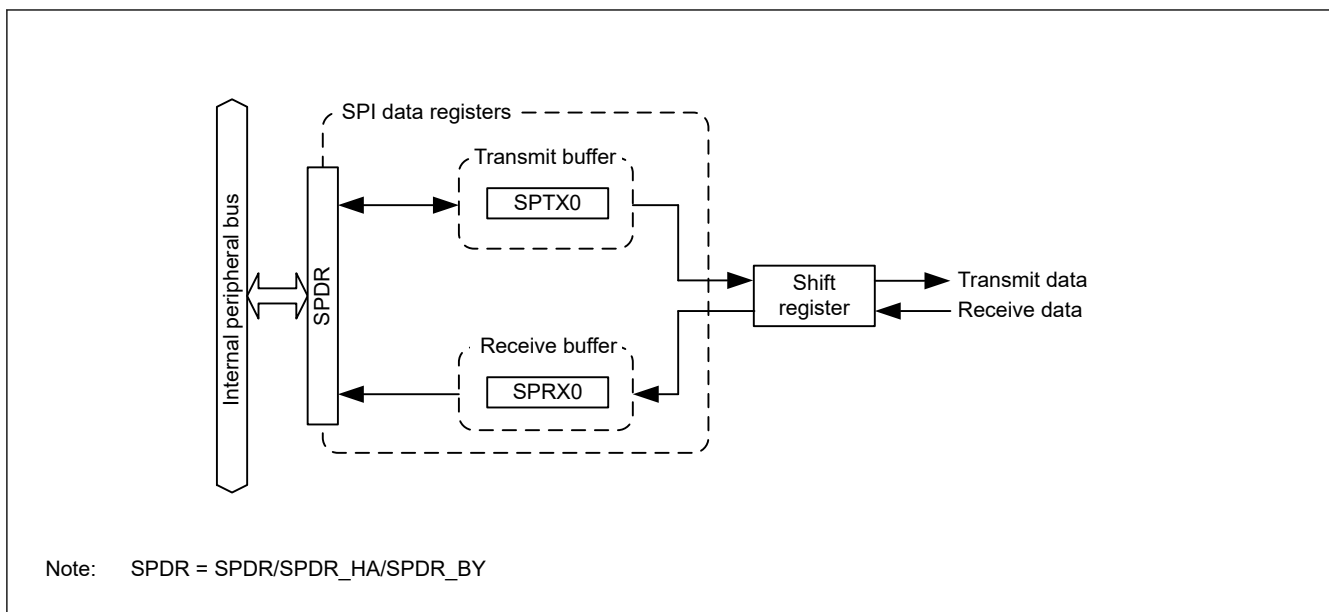
Figure 26.2 Configuration of SPDR/SPDR_HA/SPDR_BY
