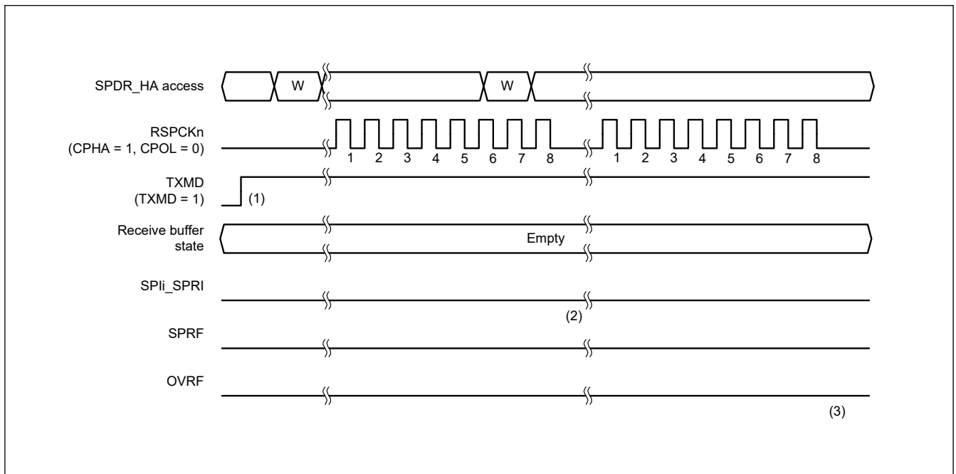
Figure 26.23 Operation example when SPCR.TXMD = 1
