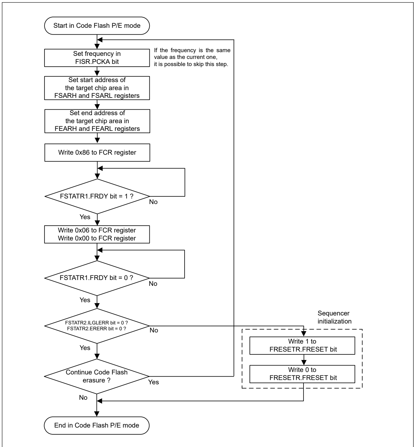
Figure 32.25 Flowchart for the code flash chip erase procedure
