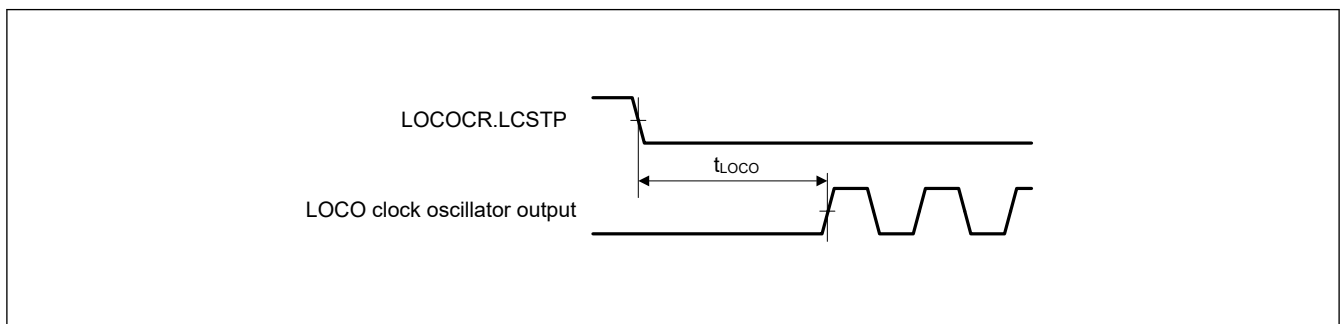
Figure 36.3 LOCO clock oscillation start timing
