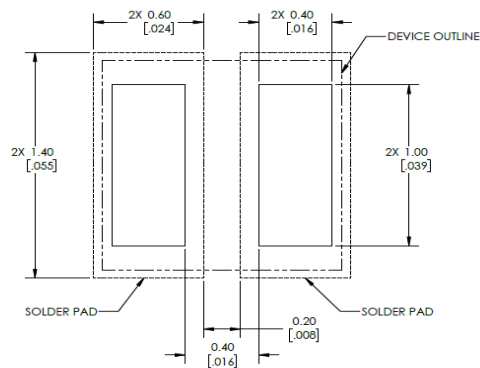
RECOMMENDED STENCIL
