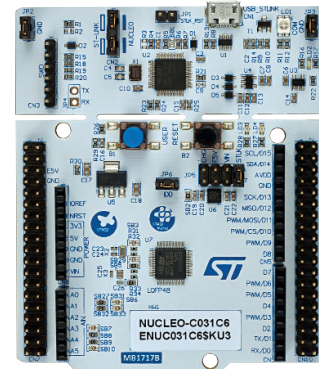
NUCLEO-C031C6 Prototyping
