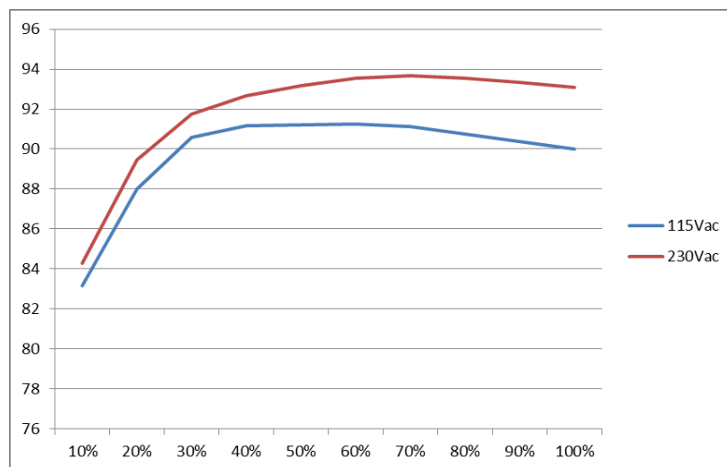
Figure 1 Typical Efficiency Curve for 24V (1200W max)
