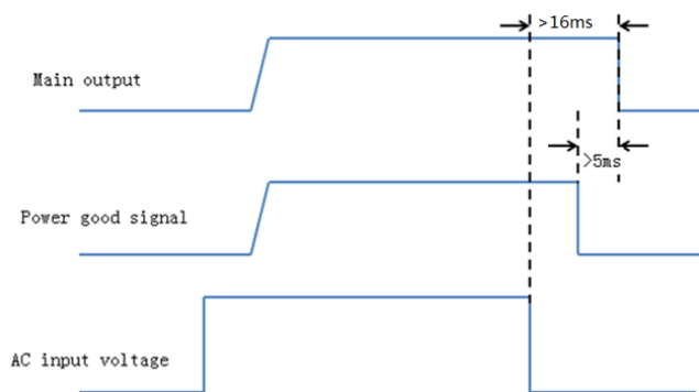
Figure 9 Power Good Time Sequence
