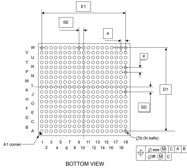
Figure 65. VFBGA361 - Outline
