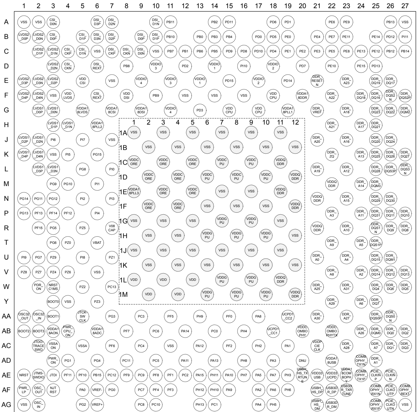
Figure 7. STM32MP25xC/F VFPGA424 pinout
