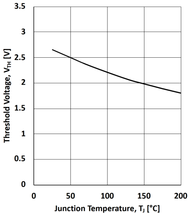
Figure 3. Threshold Voltage
