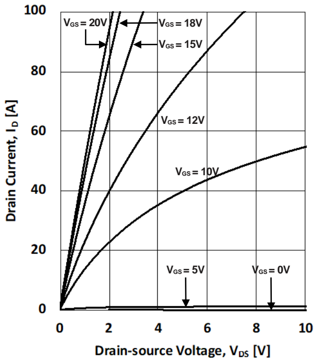
Figure 1. Output Characteristics
