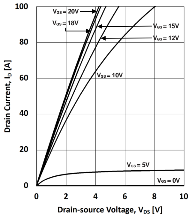
Figure 2. Output Characteristics
