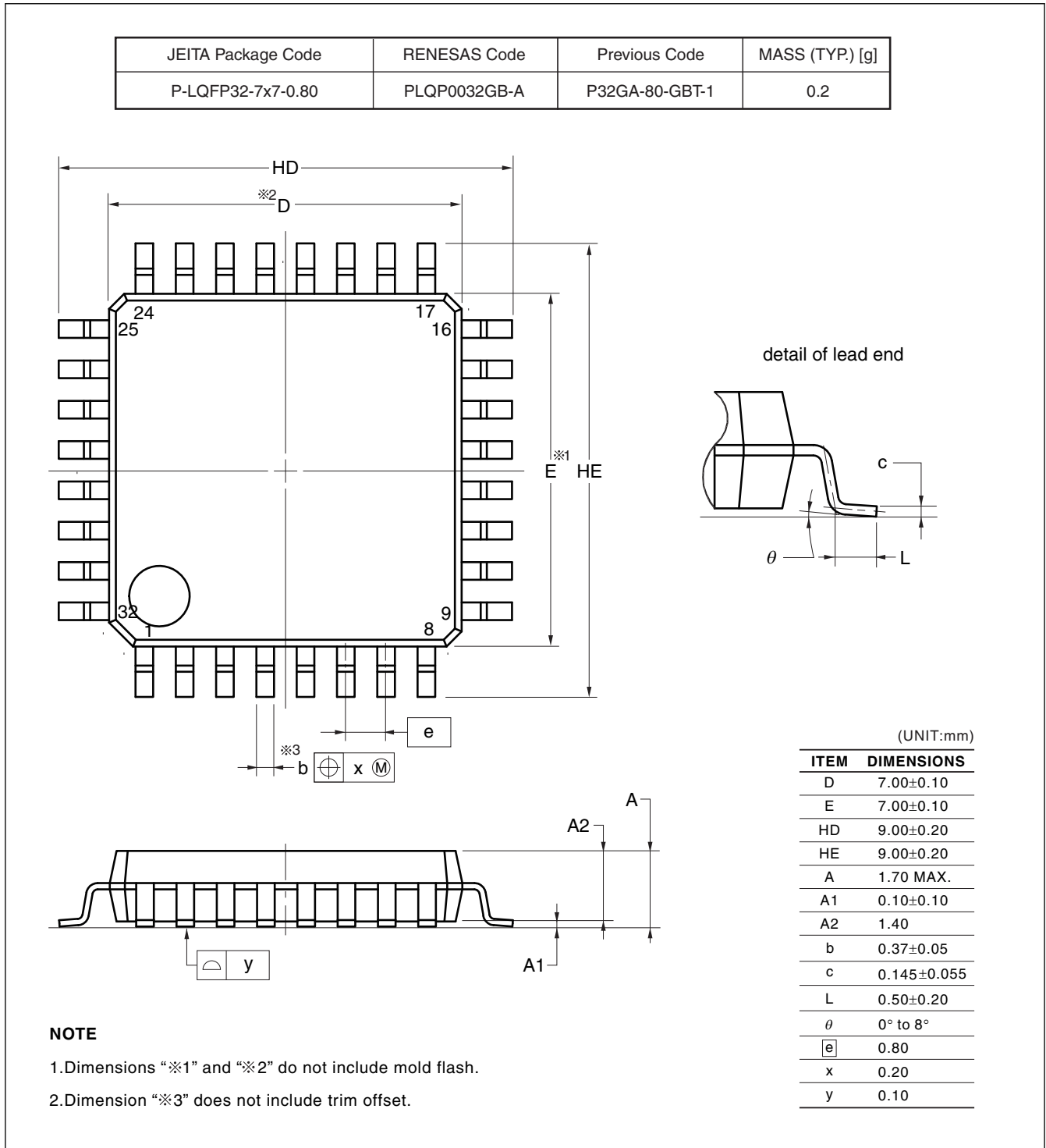
Figure 2.1 LQFP 32-pin
