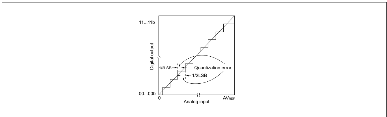
Figure 25.30 Quantization error
