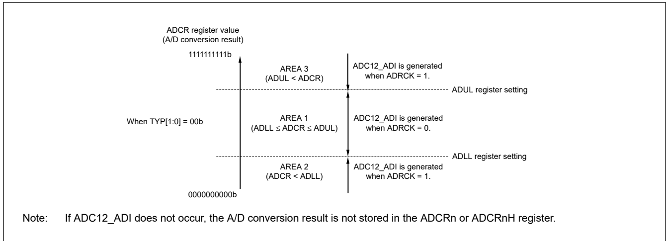
Figure 25.5 ADCRk bit interrupt signal generation range (in 10-bit resolution mode)
