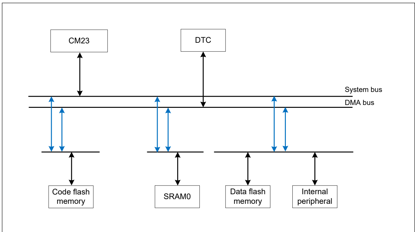
Figure 12.1 Bus configuration
