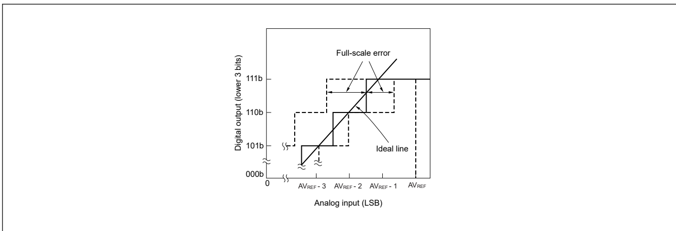
Figure 25.32 Full-scale error
