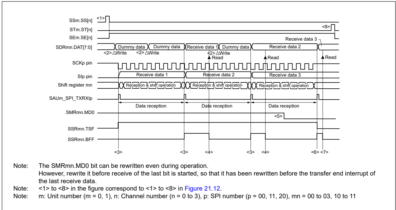
Figure 21.11 Timing of master reception (in continuous reception mode) (type 1: DCPmn[1:0] = 00b)
