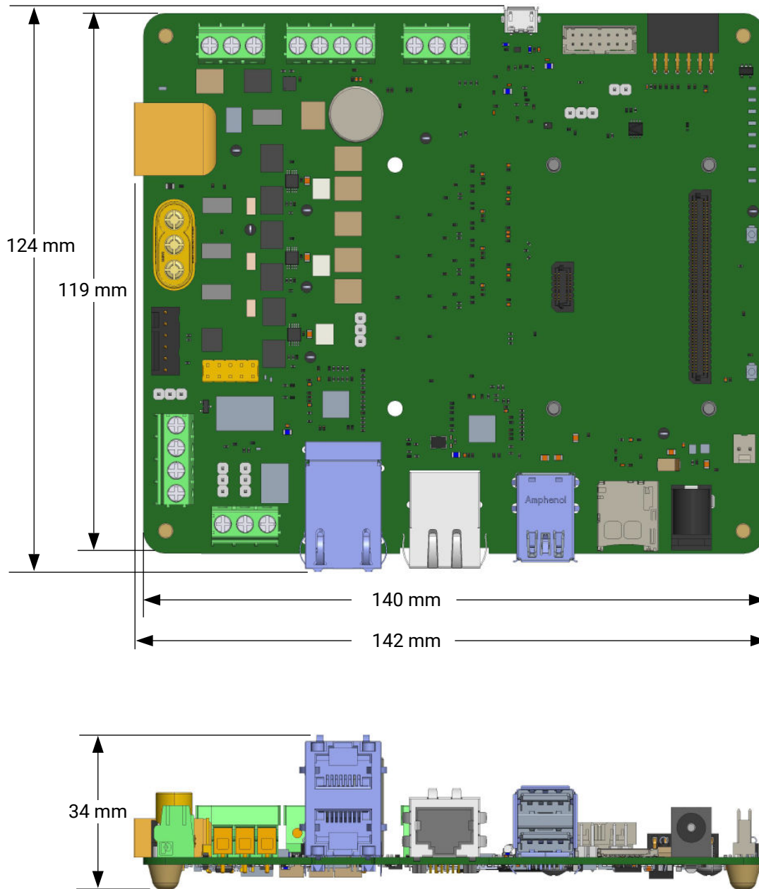
Figure 5: Kria KD240 Drives Starter Kit Carrier Card Mechanical Dimensions
