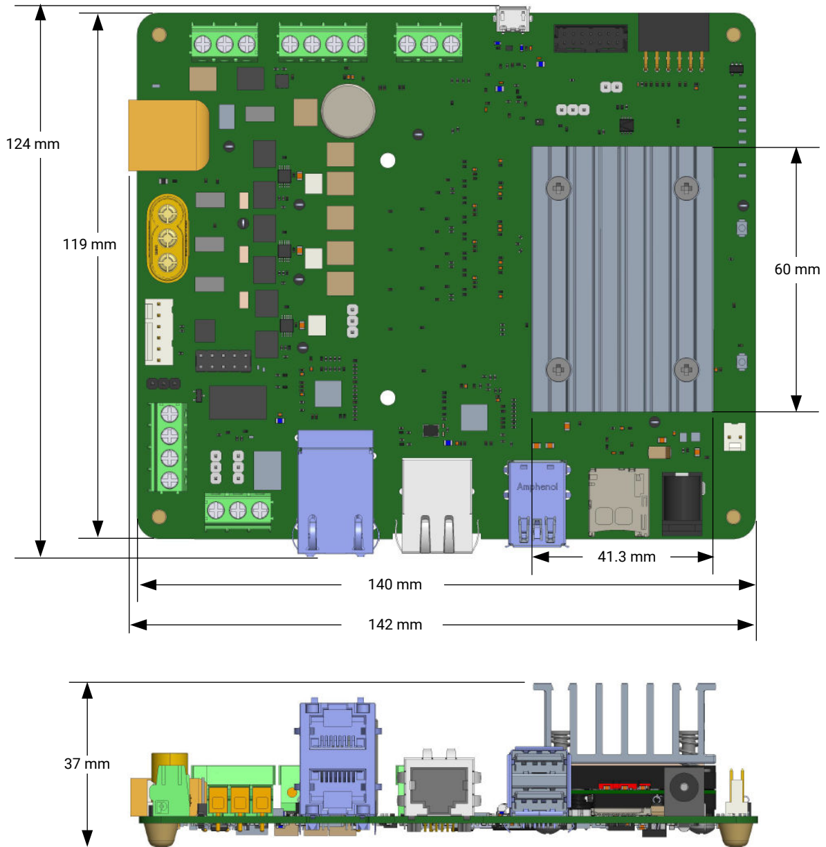
Figure 4: Kria KD240 Drives Starter Kit Mechanical Dimensions
