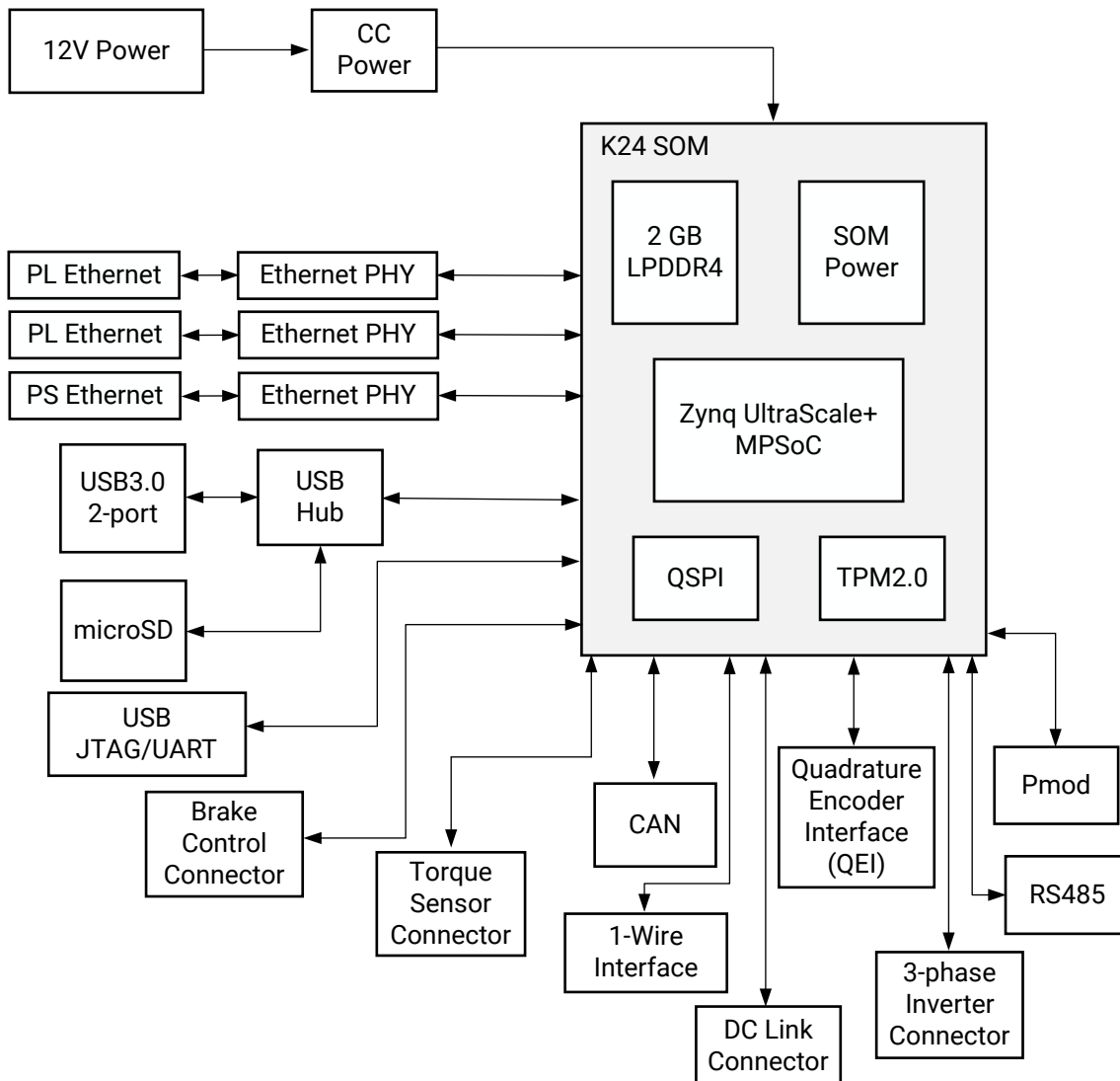
Figure 2: KD240 Starter Kit Block Diagram
