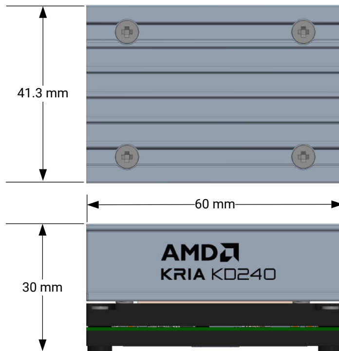
Figure 3: K24 SOM on the Kria KD240 Drives Starter Kit Mechanical Dimensions
