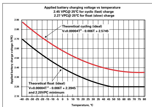
Figure 6-1: Variation of Charge Voltage with Temperature
