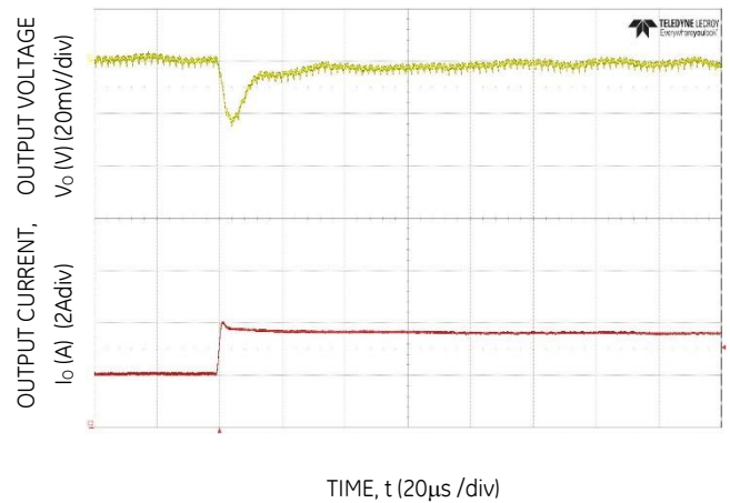
Figure 10. Transient Response to Dynamic Load Change from 50% to 100% at 12Vin, Cout=8x47µF, CTune=4.7nF, RTune=300
