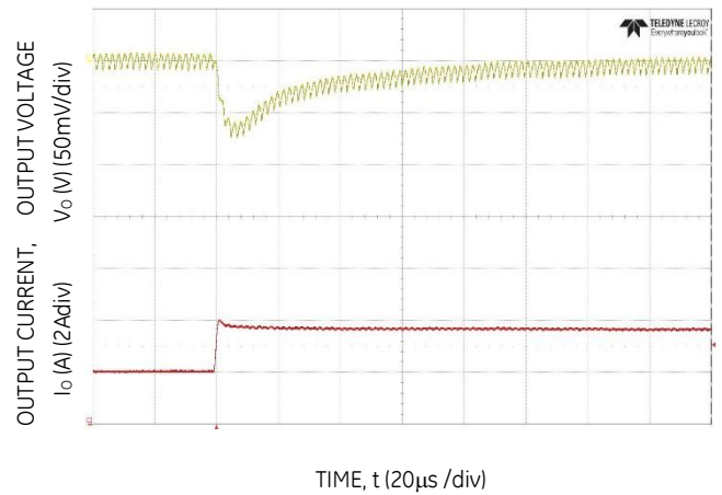
Figure 28 Transient Response to Dynamic Load Change from 50% to 100% at 12Vin, Cout=3x47uF, CTune=470pF, RTune=300
