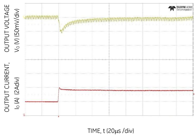
Figure 22. Transient Response to Dynamic Load Change from 50% to 100% at 12Vin, Cout=3x47uF, CTune=1.5nF, RTune=300
