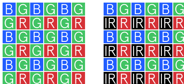
Standard Bayer RGB CFA
