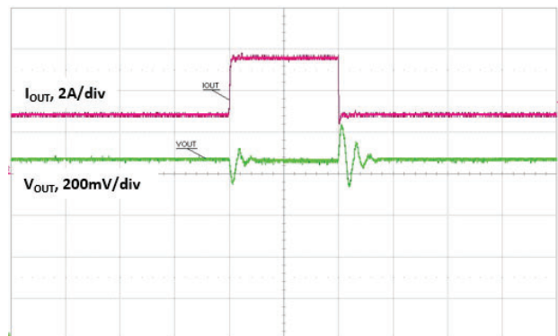
Fig. 27 - Load Transient (3 A to 6 A), Time = 100 \mu s/div
