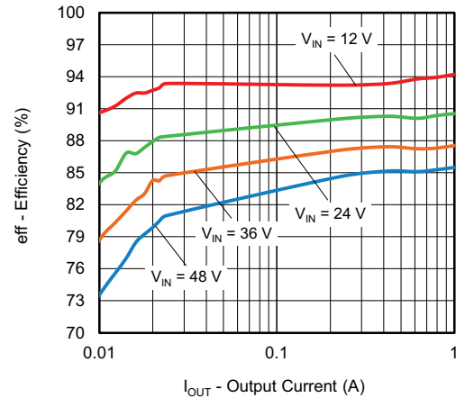
Fig. 14 - Efficiency vs. Output Current - Light Load, V_{OUT} = 5\text{ V}
