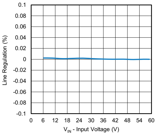
Fig. 19 - Line Regulation
