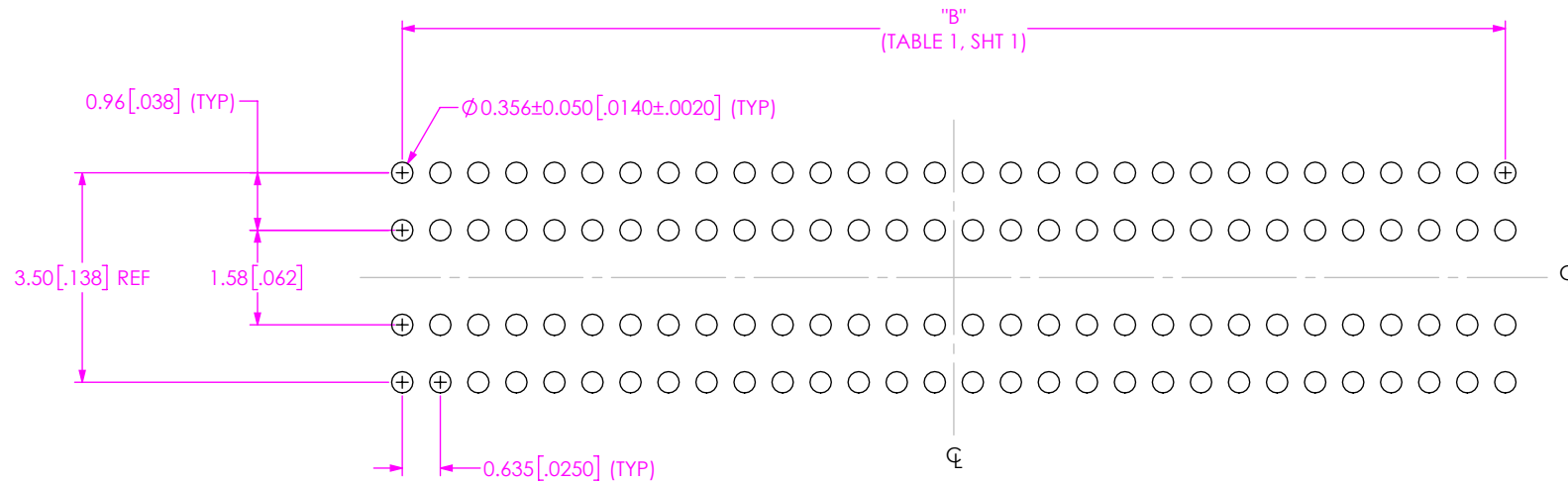
FIG 2 ADF6-30-XX.X-XXX-4-2-A STENCIL SHOWN E
