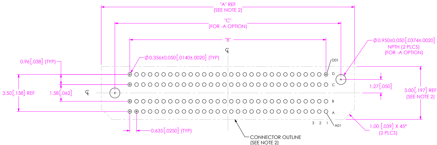
FIG 1 ADF6-30-XX.X-XXX-4-X-A SHOWN
