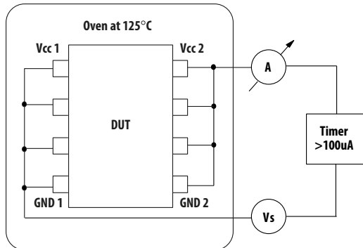
Figure 3: High Voltage Life Test Setup
