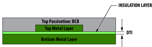
Figure 2: Magnetic and Capacitive Isolator Construction
