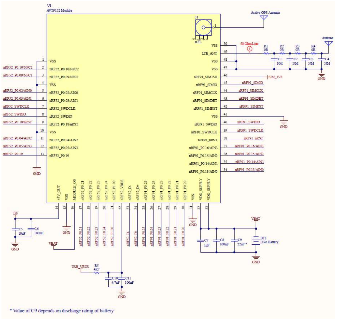
Figure 13: Reference Schematic
