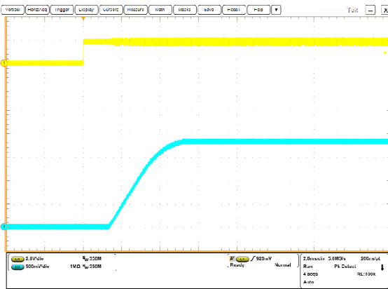
On/Off Enable Delay (Vin=5.0V, Vout=1.8V, Iout=6A, Load=400uF) Trace1=Enable, Trace2=Vout, 2 ms/div
