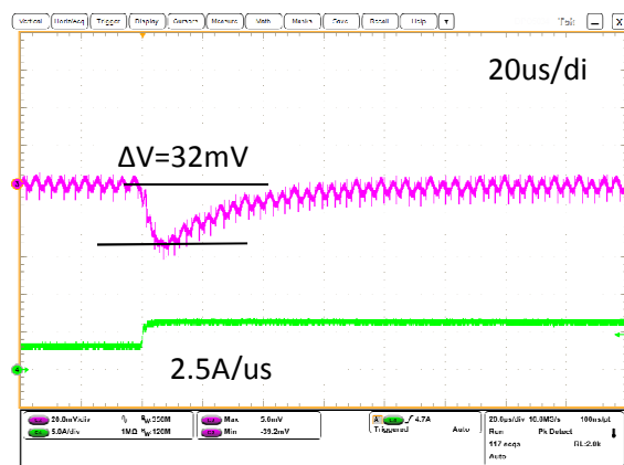
Step Load Transient Response (Vin=5.0V, Vout=1.8V, Load=400uF, Iout=3A to 6A) Trace 3=Vout, 20 mV/div, Trace 4=Iout, 5A/div.
