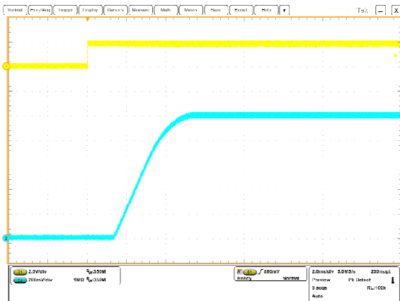
On/Off Enable Delay (Vin=5.0V, Vout=1.0V, Iout=6A, Cload=400uF) Trace1=Enable, Trace2=Vout, 2 ms/div
