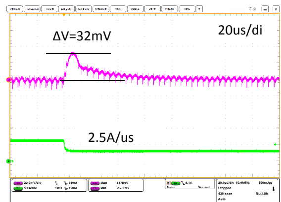
Step Load Transient Response (Vin=5.0V, Vout=1.0V, Cload=400uF, Iout=3A to 6A) Trace 3=Vout, 20 mV/div, Trace 4=Iout, 5A/div.
