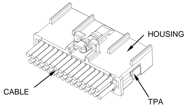
Receptacle Assembly
