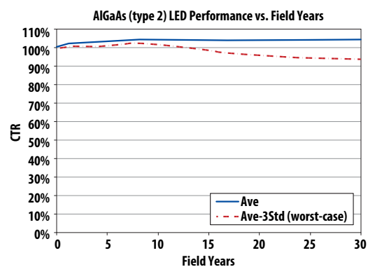
Figure 2: CTR Performance vs. Field Years for AlGaAs (Type 2) LED (Operating I_F = 5 mA, 100% Duty Cycle, T_A = 80^\circ\text{C} )
