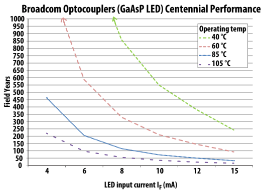
Figure 7: Centennial Performance for GaAsP LED
