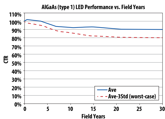
Figure 1: CTR Performance vs. Field Years for AlGaAs (Type 1) LED (Operating I_F = 16 mA, 50% Duty Cycle, T_A = 80^\circ\text{C} )
